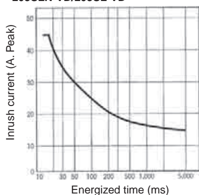
G3F-203SN-VD/203S-VD/202SN-VD/ 203SLN-VD/203SL-VD
