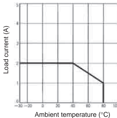
G3F-202SN-VD G3FD-102SN-VD/102S-VD
